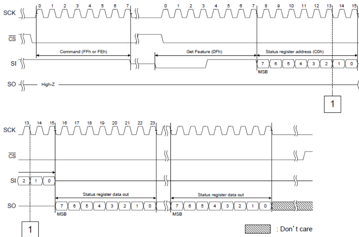
Figure 20. Reset Timing
