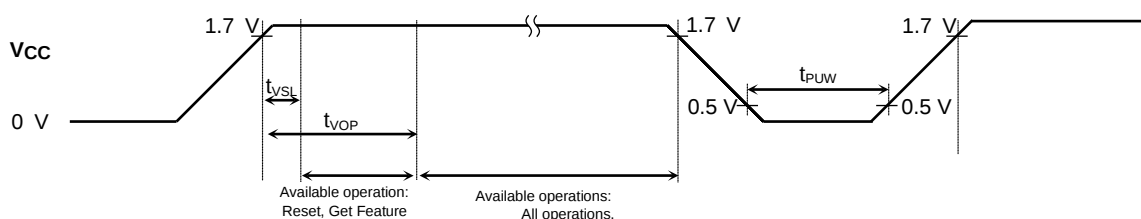
Figure 11. Power ON/OFF Sequence
